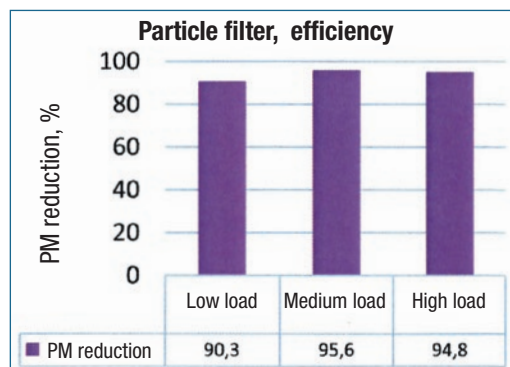
Figure 2: Cleaning efficiency of the particle filter of three load point, (%)
