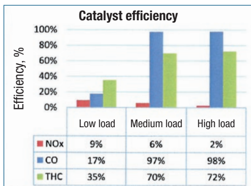
Figure 1: Catalyst efficiency of the reduction of THC, CO and NOx, (%)
